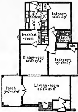
First-floor Plan
